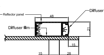
LED holder+soft silicone diffuser
