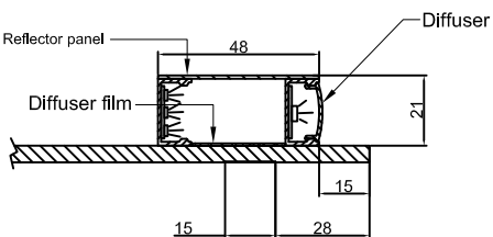
LED holder+soft silicone diffuser
